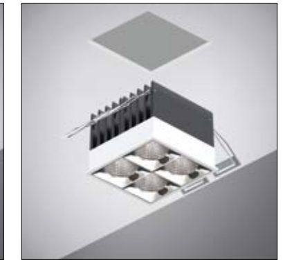
Task 319 downlight cartongesso L8x8 - 18W
